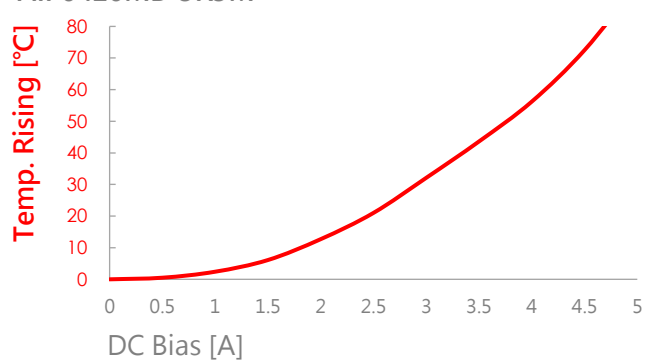
AIP0420MB-3R3M
