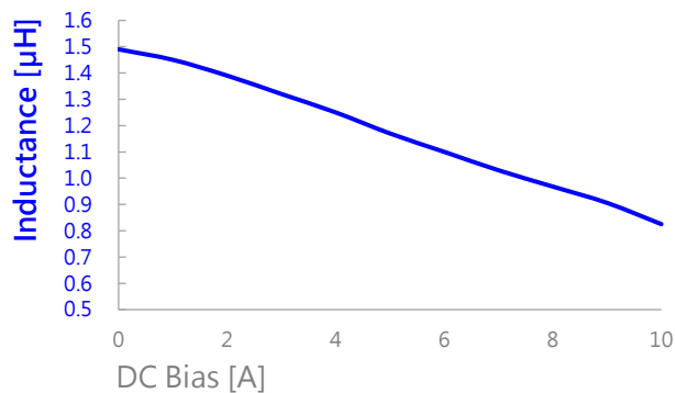
AIP0420MB-1R5M
