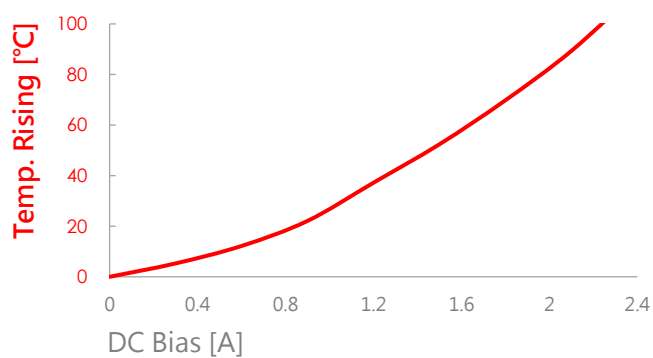
AIP0420MB-220M
