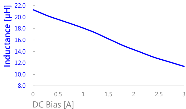
AIP0420MB-220M
