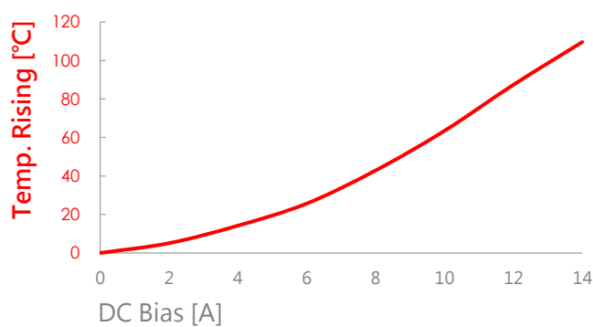
AIP0420MB-R68M
