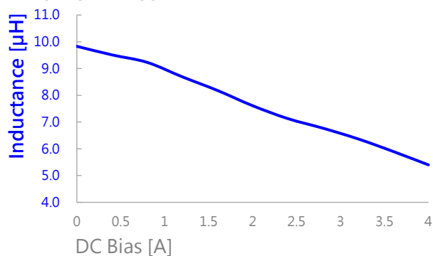
AIP0420MB-100M
