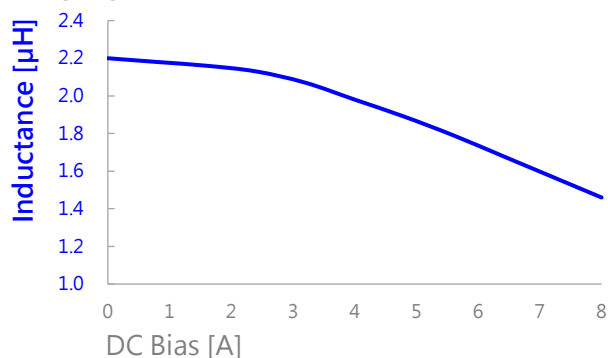
AIP0420MB-2R2M
