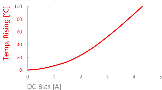
AIP0420MB-6R8M
