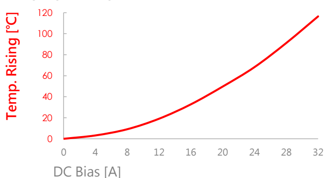
AIP0420MB-R10M
