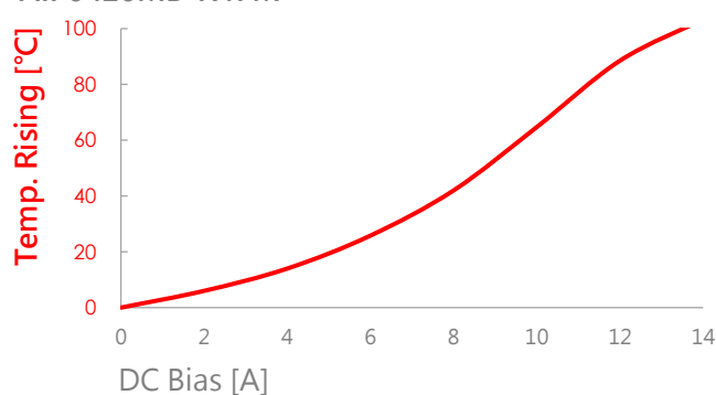
AIP0420MB-R47M
