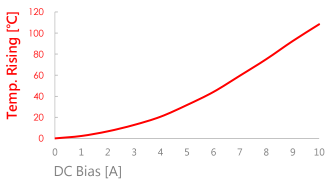
AIP0420MB-1R5M
