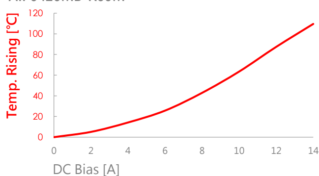
AIP0420MB-R60M
