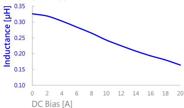
AIP0420MB-R33M
