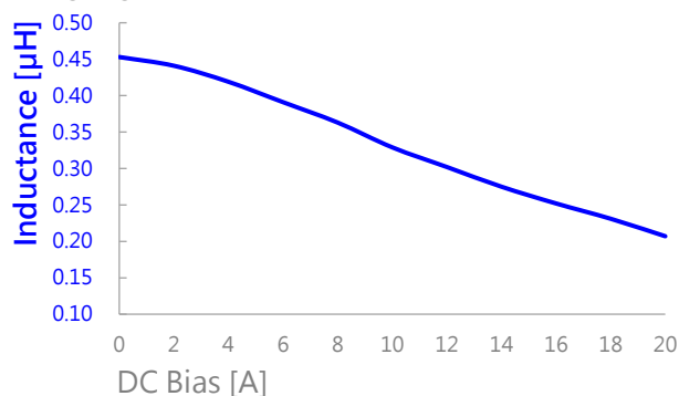
AIP0420MB-R47M
