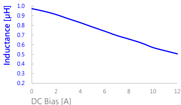
AIP0420MB-1R0M
