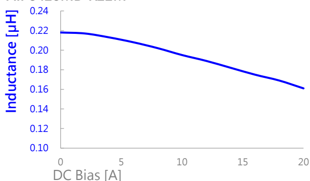
AIP0420MB-R22M
