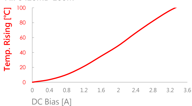
AIP0420MB-100M
