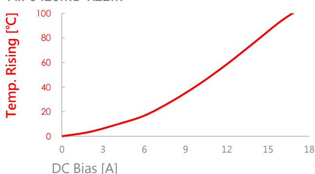
AIP0420MB-R22M
