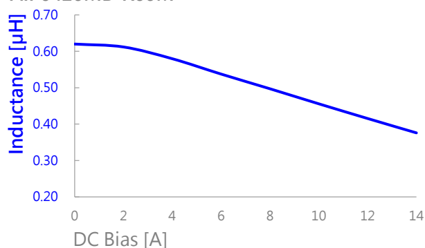
AIP0420MB-R60M
