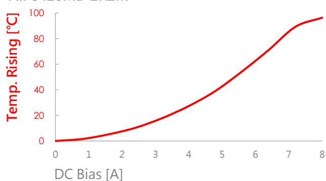
AIP0420MB-2R2M
