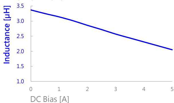
AIP0420MB-3R3M
