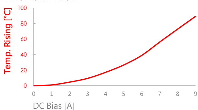
AIP0420MB-1R0M
