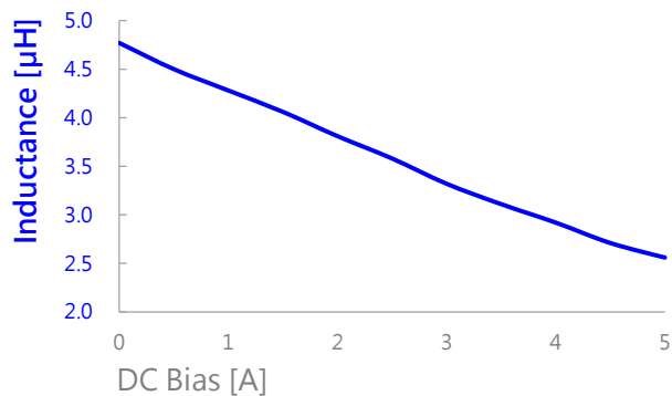
AIP0420MB-4R7M
