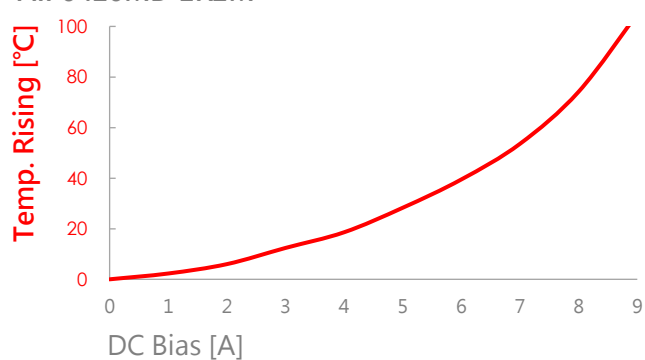
AIP0420MB-1R2M
