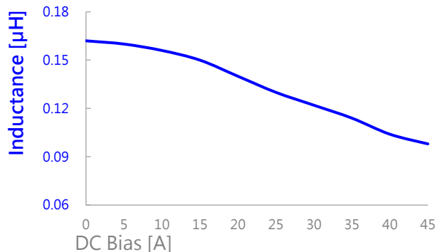
AIP0630MB-R15M
