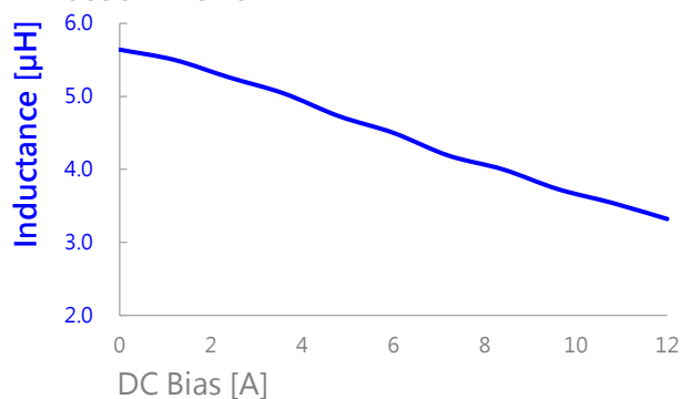
AIP0630MB-5R6M
