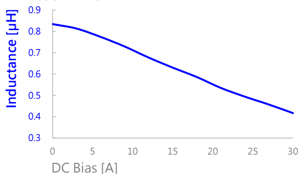
AIP0630MB-R82M
