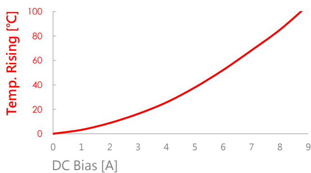
AIP0630MB-6R8M
