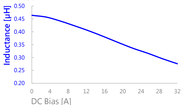
AIP0630MB-R47M
