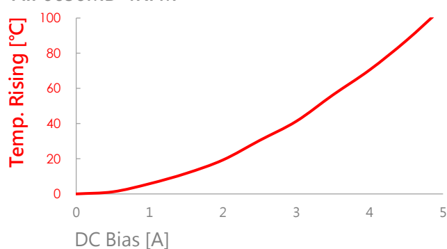
AIP0630MB-4R7M
