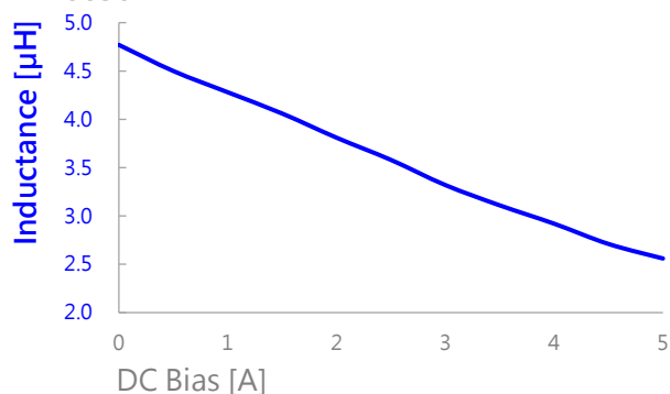
AIP0630MB-4R7M
