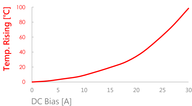
AIP0630MB-R33M
