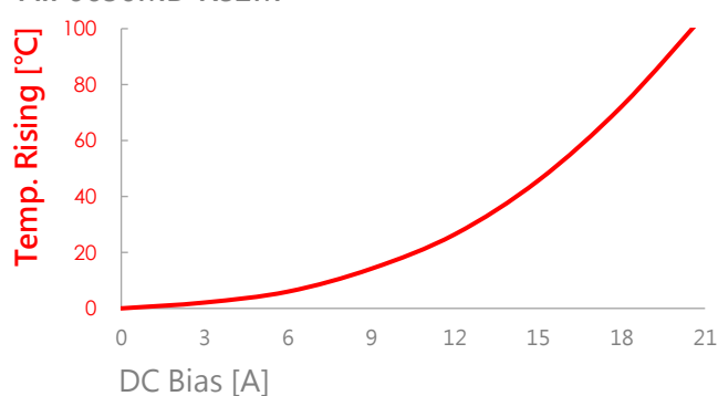
AIP0630MB-R82M
