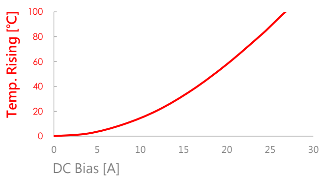
AIP0630MB-R68M
