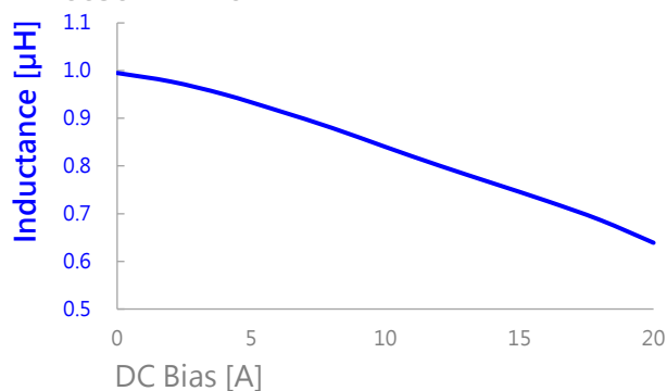
AIP0630MB-1R0M
