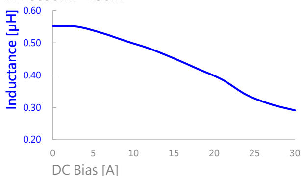
AIP0630MB-R56M
