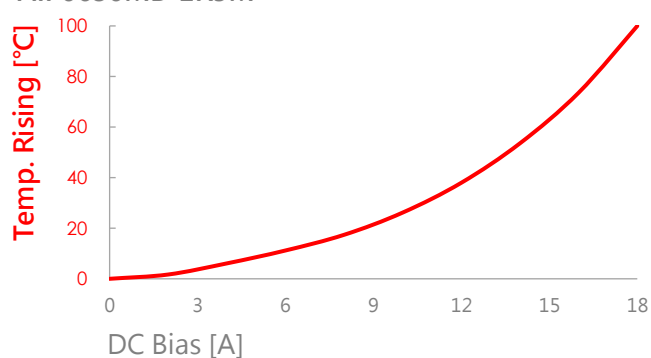
AIP0630MB-1R5M
