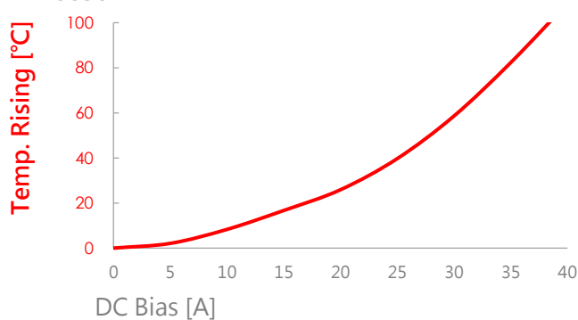
AIP0630MB-R22M
