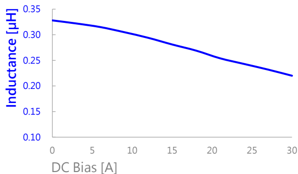
AIP0630MB-R33M
