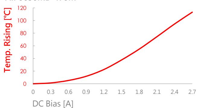
AIP0630MB-470M
