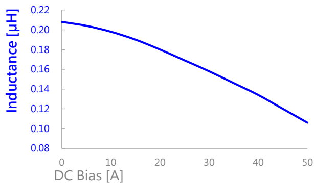
AIP0630MB-R22M
