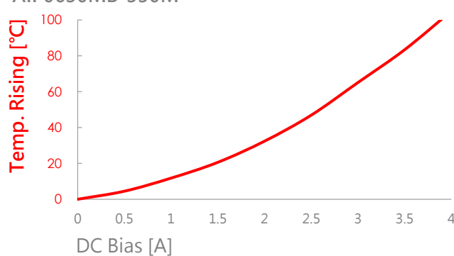
AIP0630MB-330M
