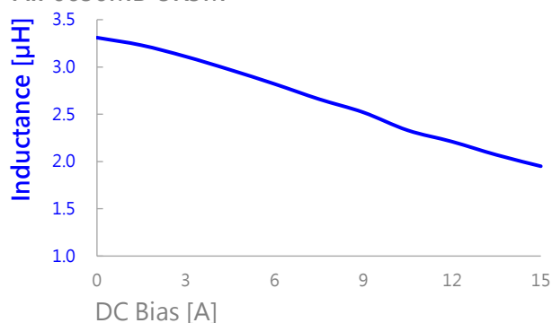
AIP0630MB-3R3M
