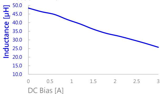
AIP0630MB-470M
