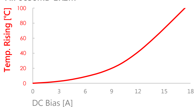
AIP0630MB-1R2M
