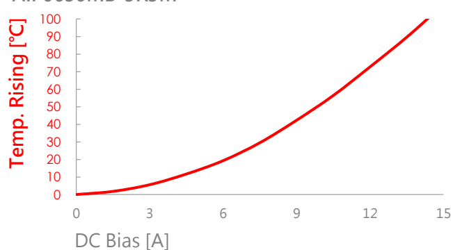
AIP0630MB-3R3M
