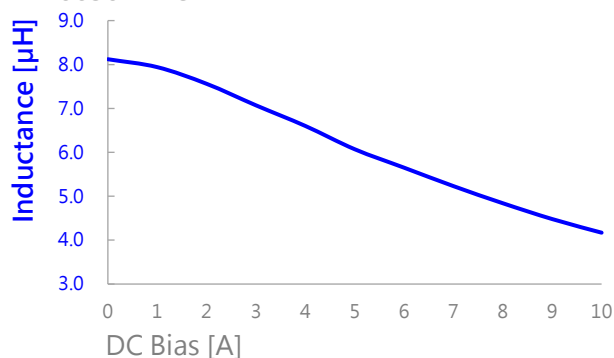
AIP0630MB-8R2M
