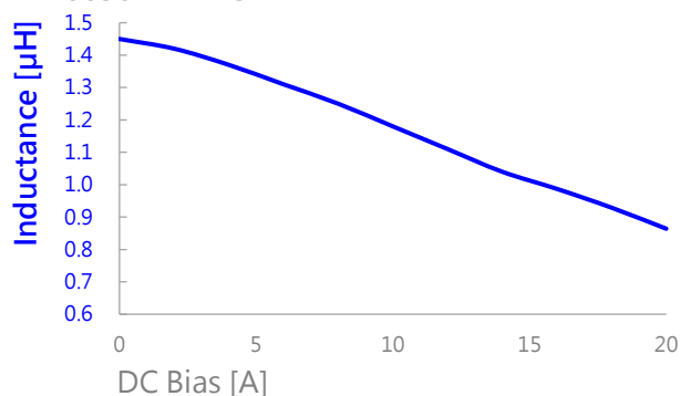
AIP0630MB-1R5M
