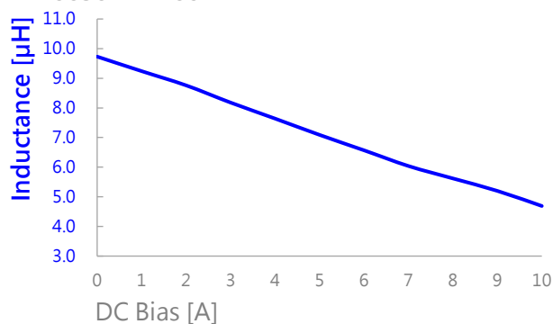
AIP0630MB-100M
