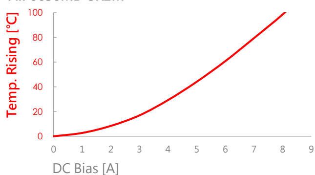
AIP0630MB-8R2M
