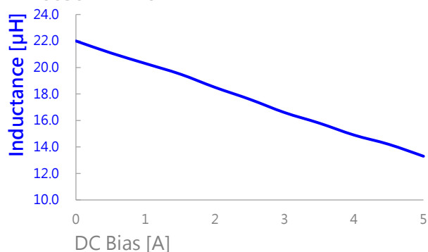
AIP0630MB-220M
