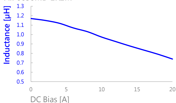
AIP0630MB-1R2M
