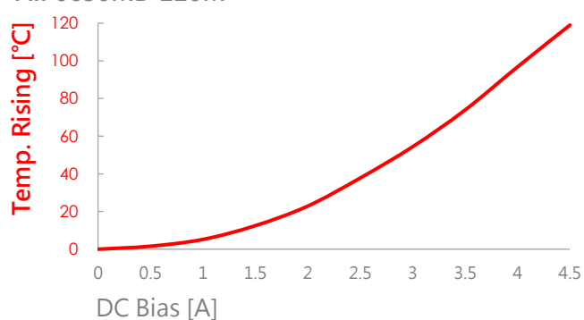
AIP0630MB-220M
