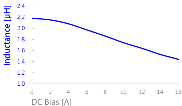
AIP0630MB-2R2M
