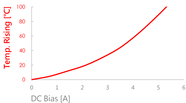
AIP0630MB-150M
