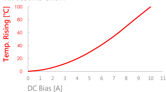
AIP0630MB-5R6M
