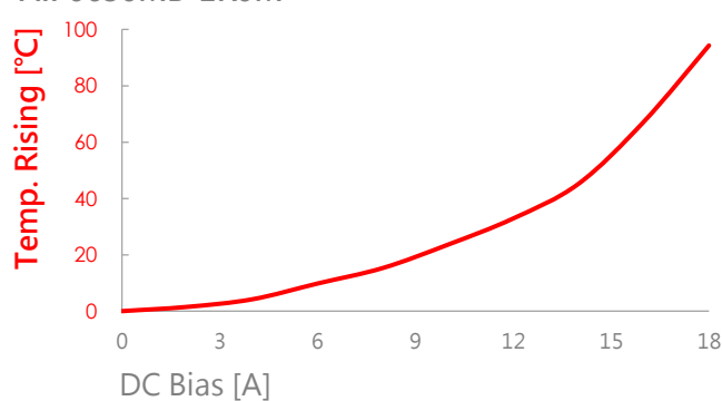
AIP0630MB-1R0M
