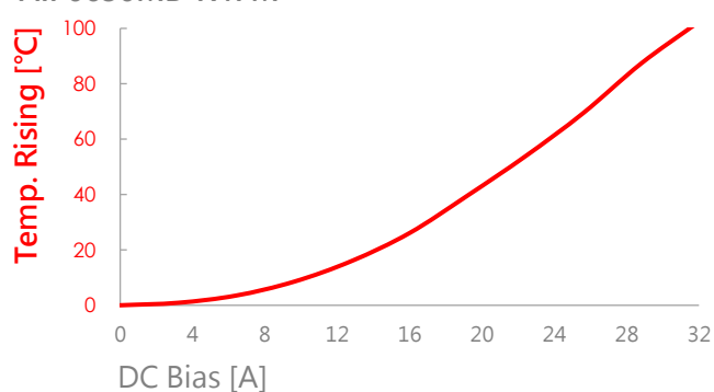
AIP0630MB-R47M
