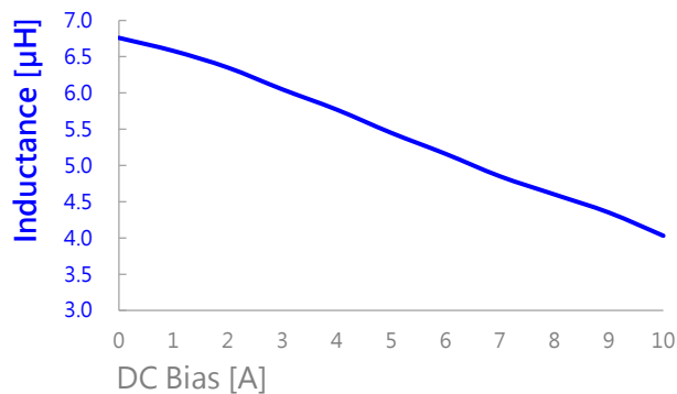
AIP0630MB-6R8M
