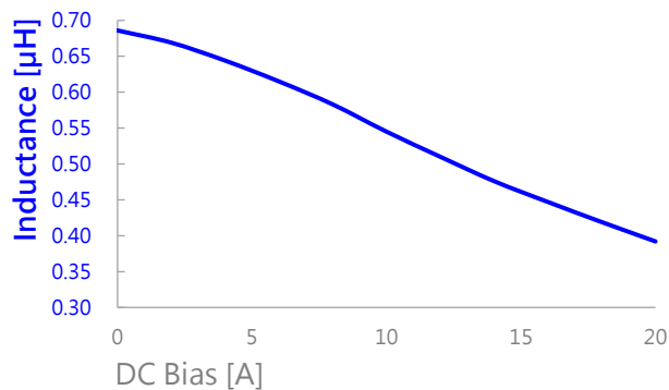
AIP0630MB-R68M
